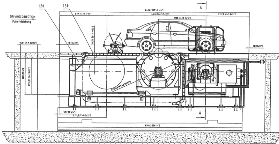
AVL road simulator on support foundation at Toyota facility in Ann Arbor, MI.
